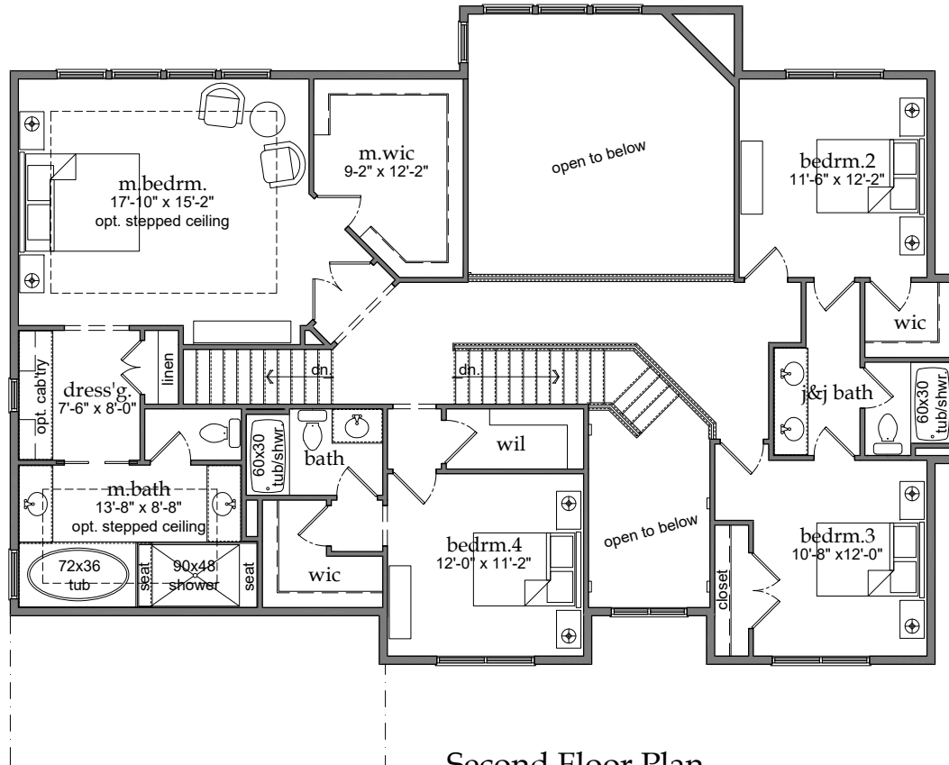
Second Floor Plan 8'-0" clg. ht. (unless noted other)
